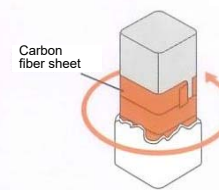
Reinforcement by wrapping with continuous carbon fiber sheet
