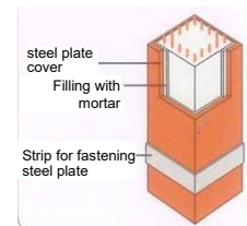
Reinforcement by covering with steel plates
